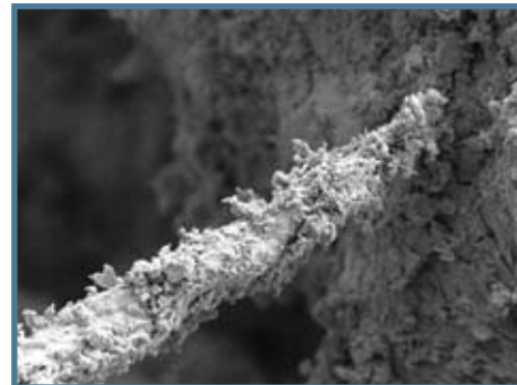
FIGURE F: UltraFiber 500® in concrete after 4.5 years
