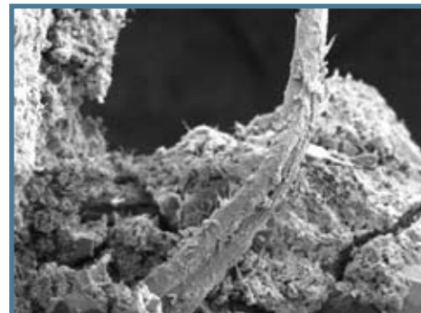
FIGURE G: UltraFiber 500® in concrete after 4.5 years
